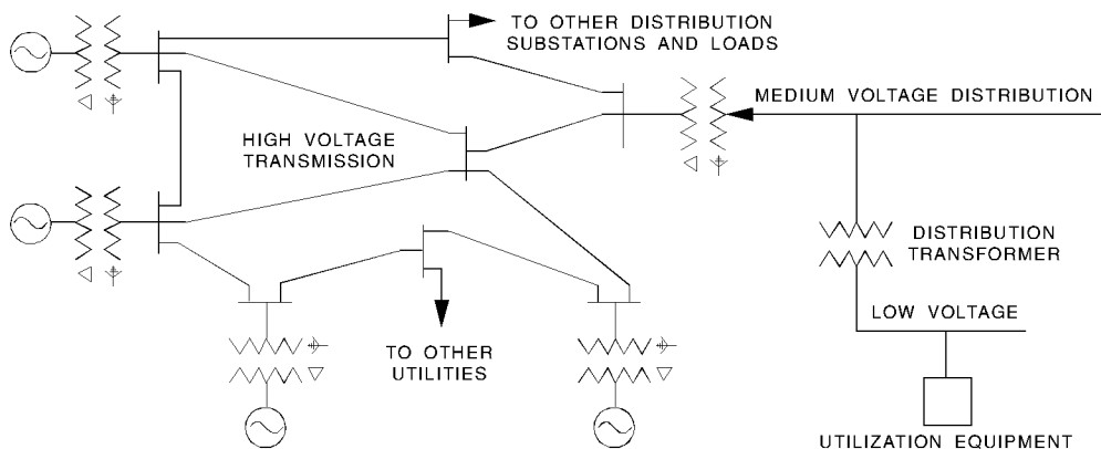
Figure 3-2—Typical utility generation, transmission and distribution system
