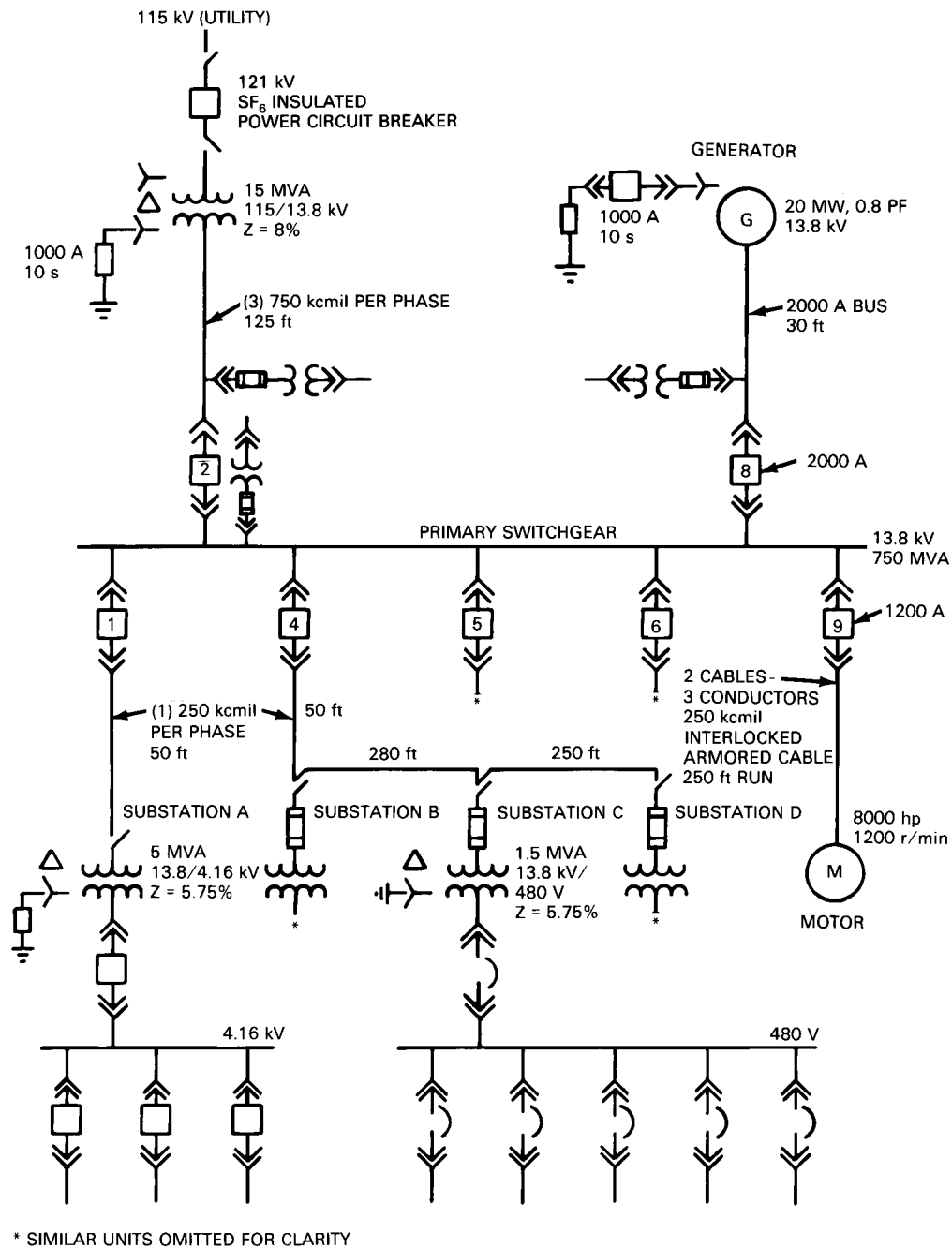
Figure 16-1—One-line diagram
